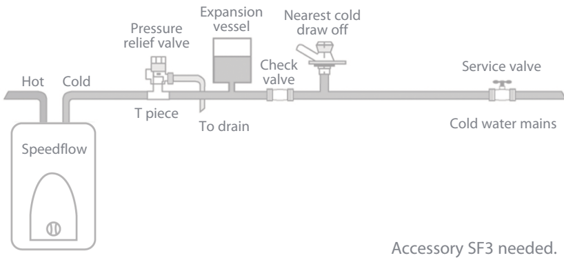
DIAGRAM C - Pressure below 4.2 bar and cold water draw off nearby
