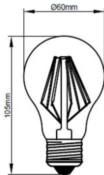
KFLM07GLS/E27-CLR
