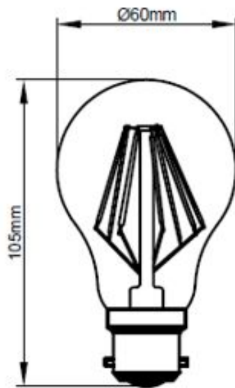
KFLM07GLS/B22-CLR
