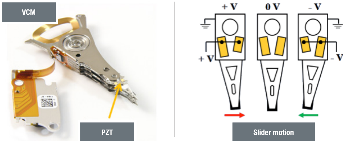
Figure 4. VCM and PZT loops work together
